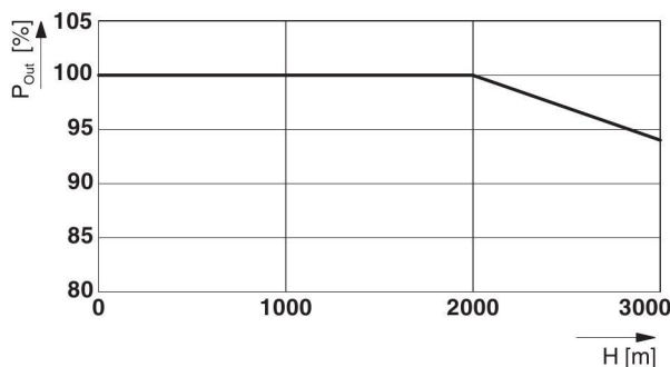
Figure 26 Altitude-dependent derating
