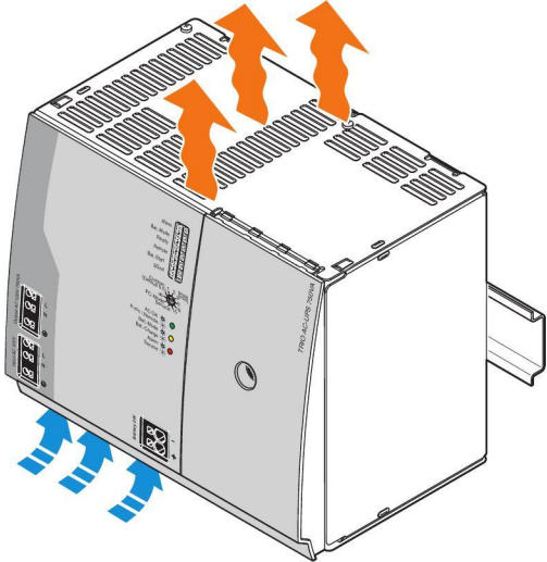
Figure 4 Convection
