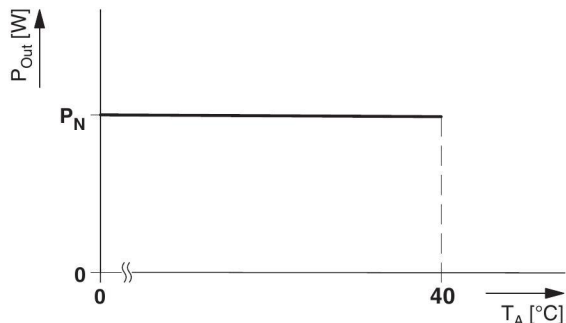
Figure 25 Temperature-dependent derating
