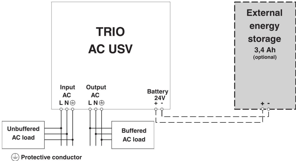
Figure 10 Schematic design
