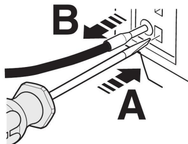
Figure 13 Release connecting cable (push-in connection technology)
